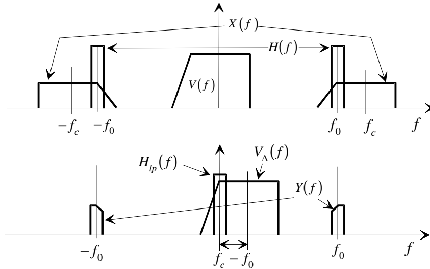
Figure C.2—Example signal spectra and filter characteristic
